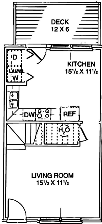
TOWNHOUSE Middle Floor
